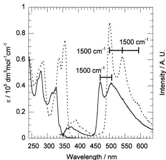
Figure 2. Absorption (left) and Emission (right) spectra of 2 (—) and 3 (----) in CH 2 Cl 2 purged N 2 at room temperature. Emission spectrum was detected upon excitation at 328 nm.
