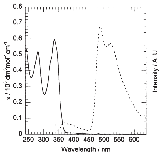
Figure 1. Absorption (—) and Emission (----) spectra of 1 in MeOH purged N 2 at room temperature. Emission spectrum was detected upon excitation at 328 nm.
